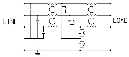
SCHEMATIC
