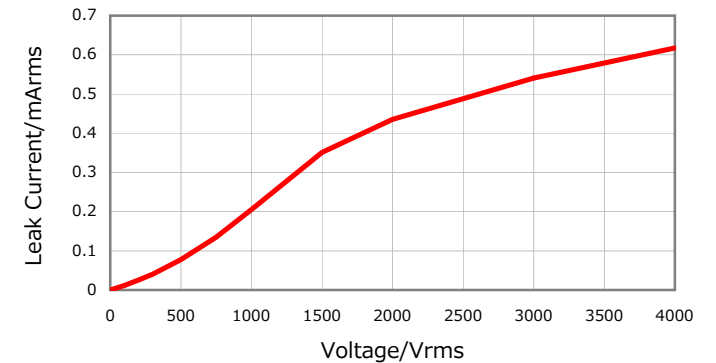
Leak Current
